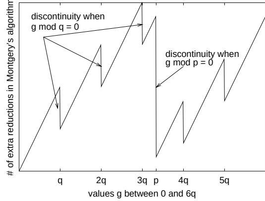
Figure 1: Number of extra reductions in a Montgomery reduction as a function (equation 1) of the input g .
